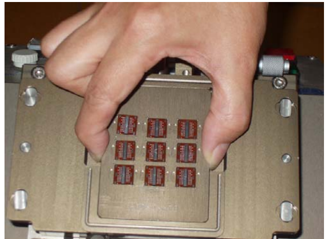
迴焊
