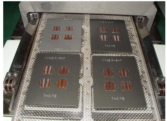
迴焊
