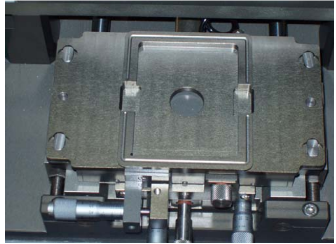
置放主模具槽
