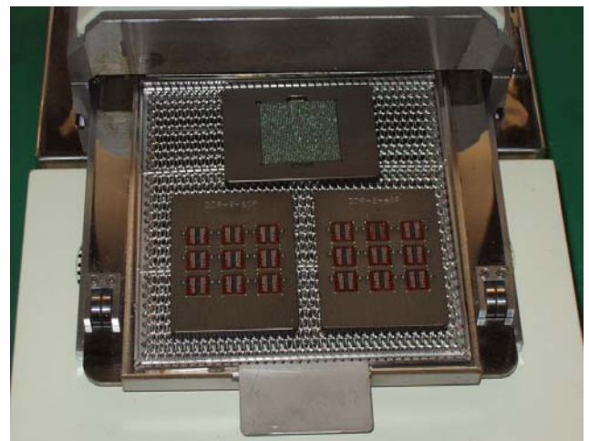
迴焊
