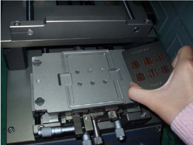
子內模具置放主模具槽
